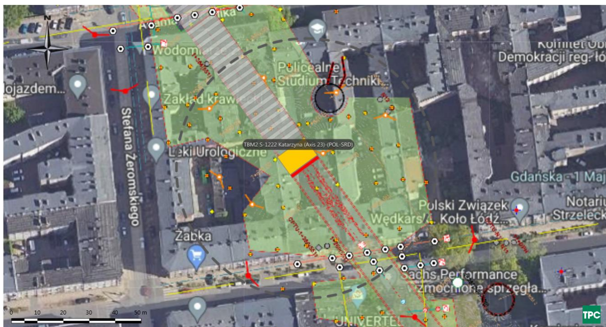
Figure 1-2 Plan view of TBM Position on 10/09/2024
