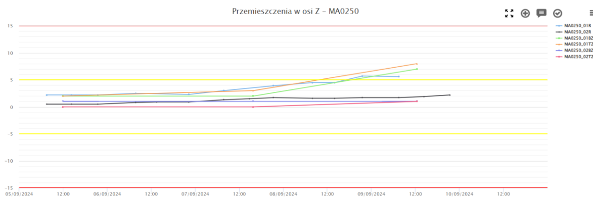
Figure 6-13 Settlement of building MA0250 - Geoscope
